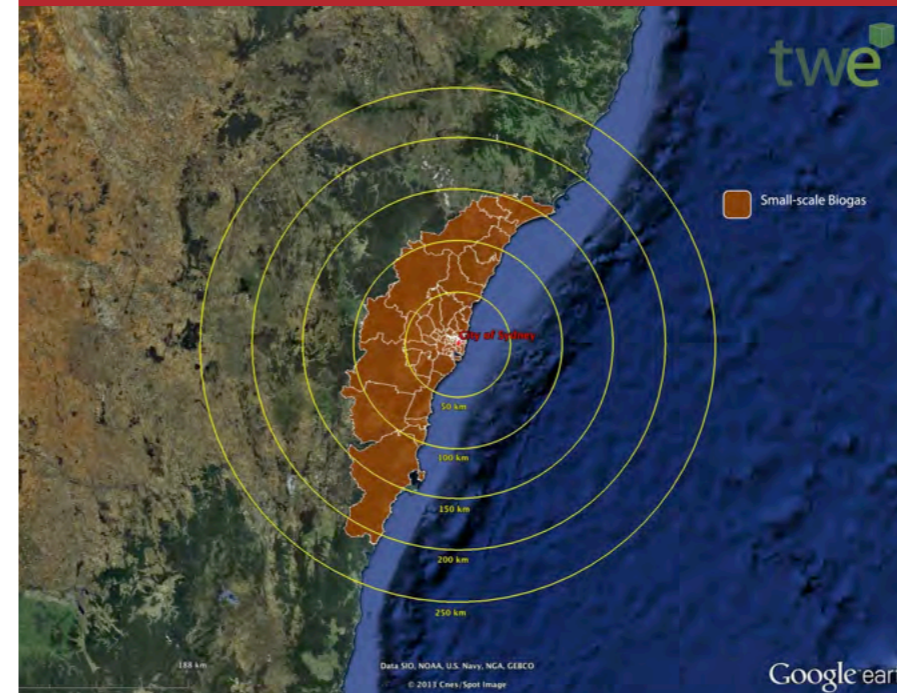
FIGURE 32: SMALL-SCALE BIOGAS – FEEDSTOCK RESOURCE CATCHMENTS (SOURCE: TALENT WITH ENERGY)
