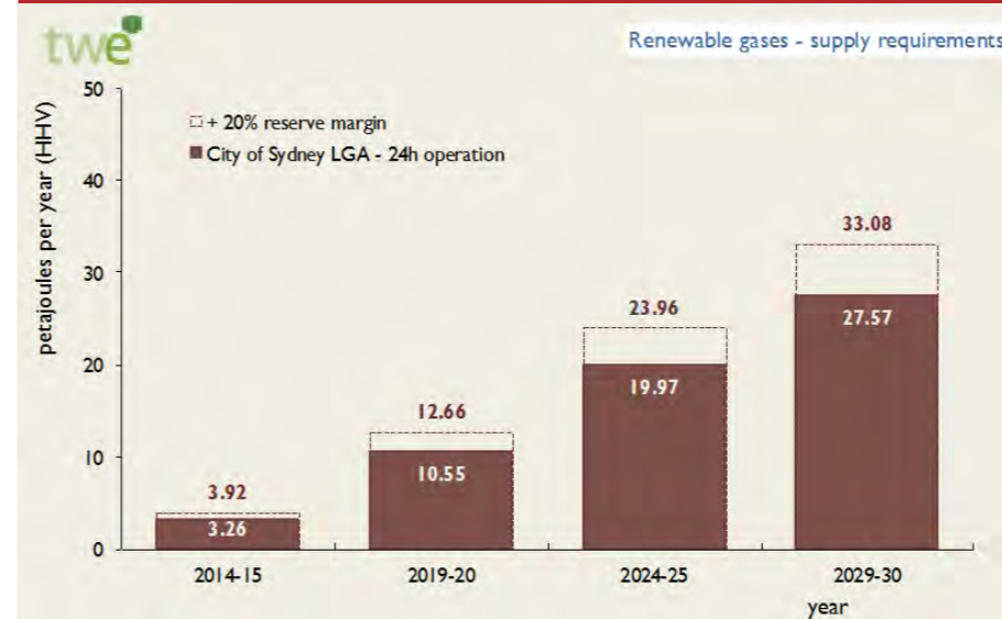
FIGURE 46: RENEWABLE GAS – SUPPLY REQUIREMENT (SOURCE: TALENT WITH ENERGY)
