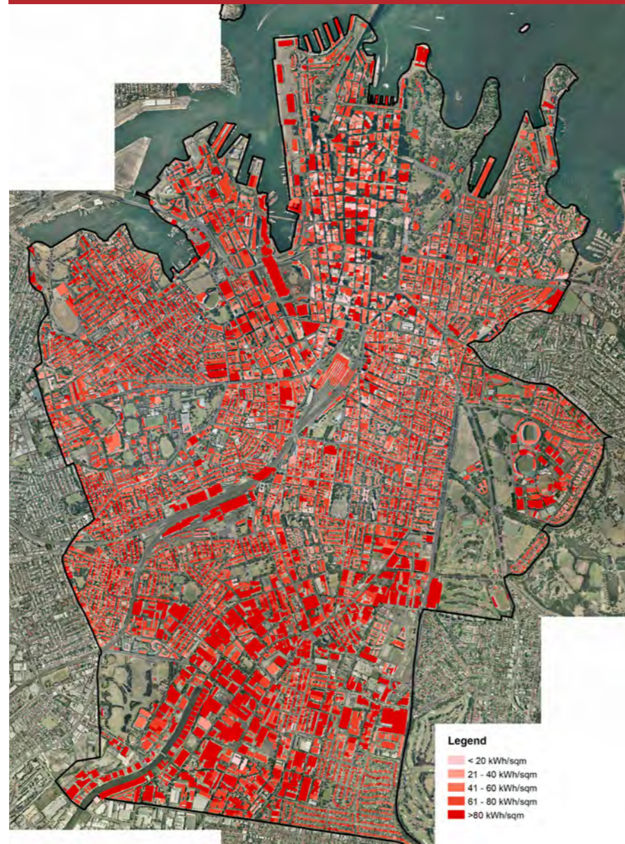
FIGURE 16: POTENTIAL BUILDINGS FOR SOLAR PV (SOURCE: ARUP)
