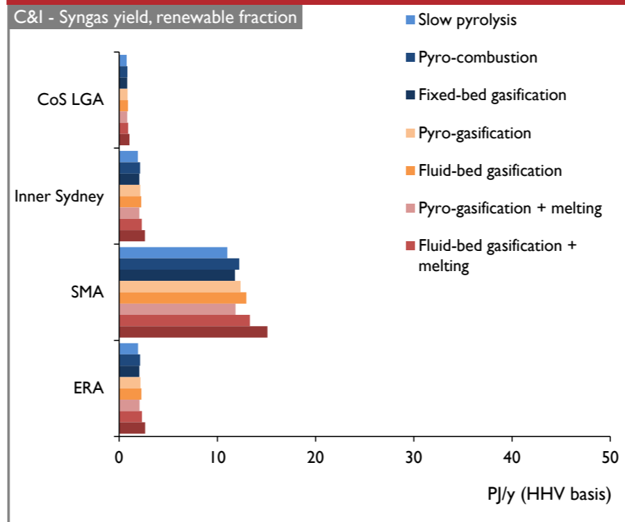
FIGURE 29: C&I – SYNGAS YIELD, RENEWABLE FRACTION PJ/Y – HHV (SOURCE: TALENT WITH ENERGY)
